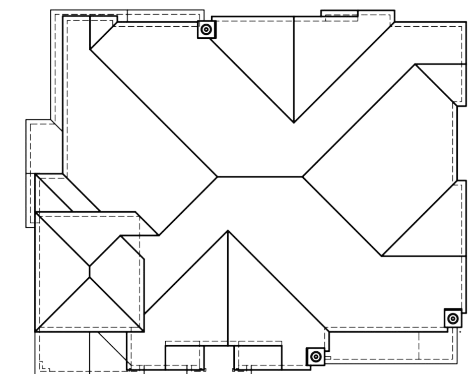
ROOF PLAN
