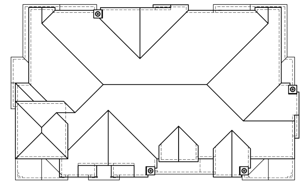
ROOF PLAN 4:12 PITCH EAVE: 12" RAKE: TIGHT
