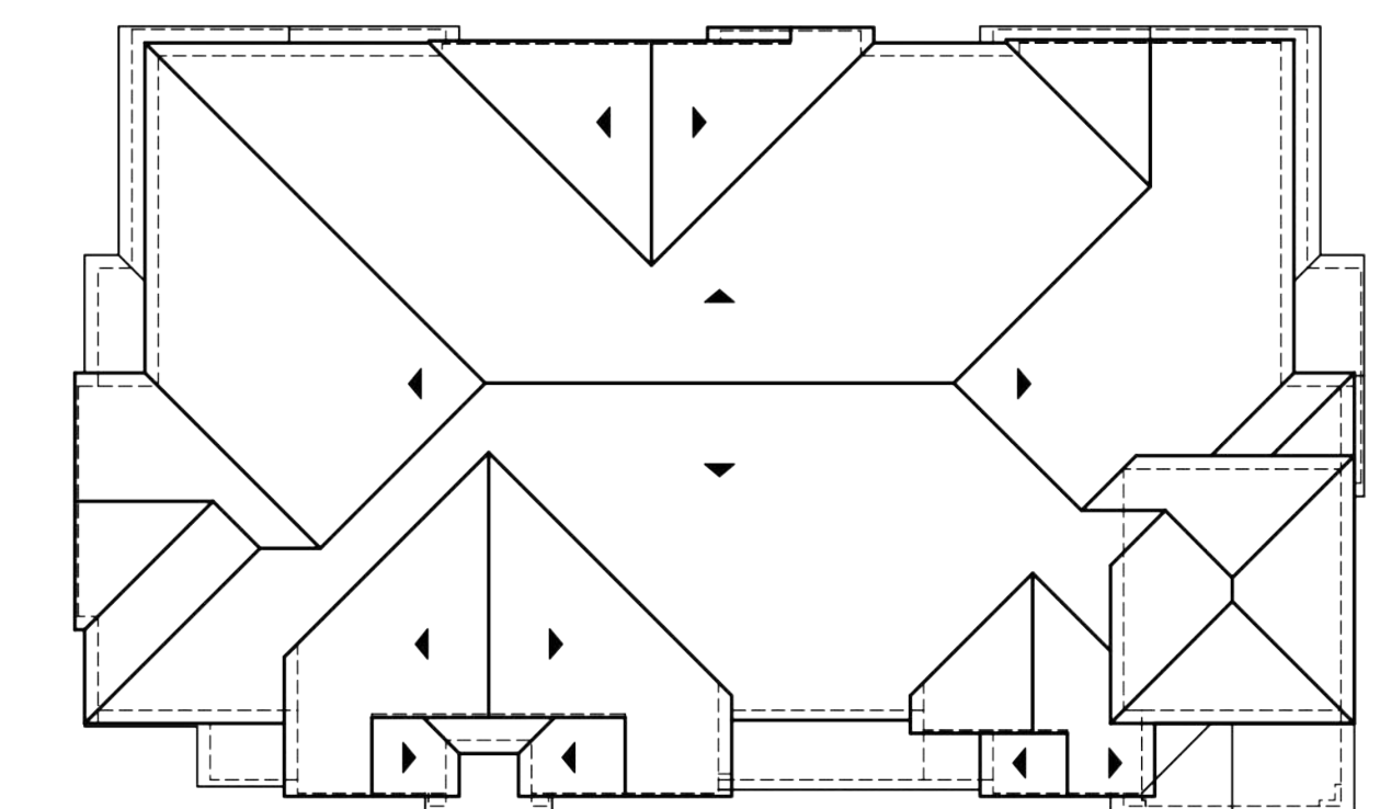
ROOF PLAN 4:12 PITCH U.N.O. EAVE: 12" RAKE: 3"
