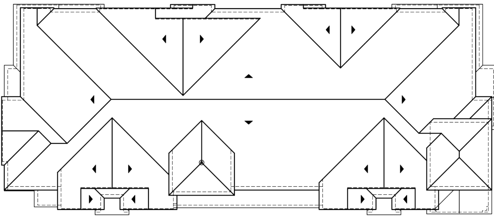
ROOF PLAN 3:12 PITCH EAVE: 12" RAKE: TIGHT
