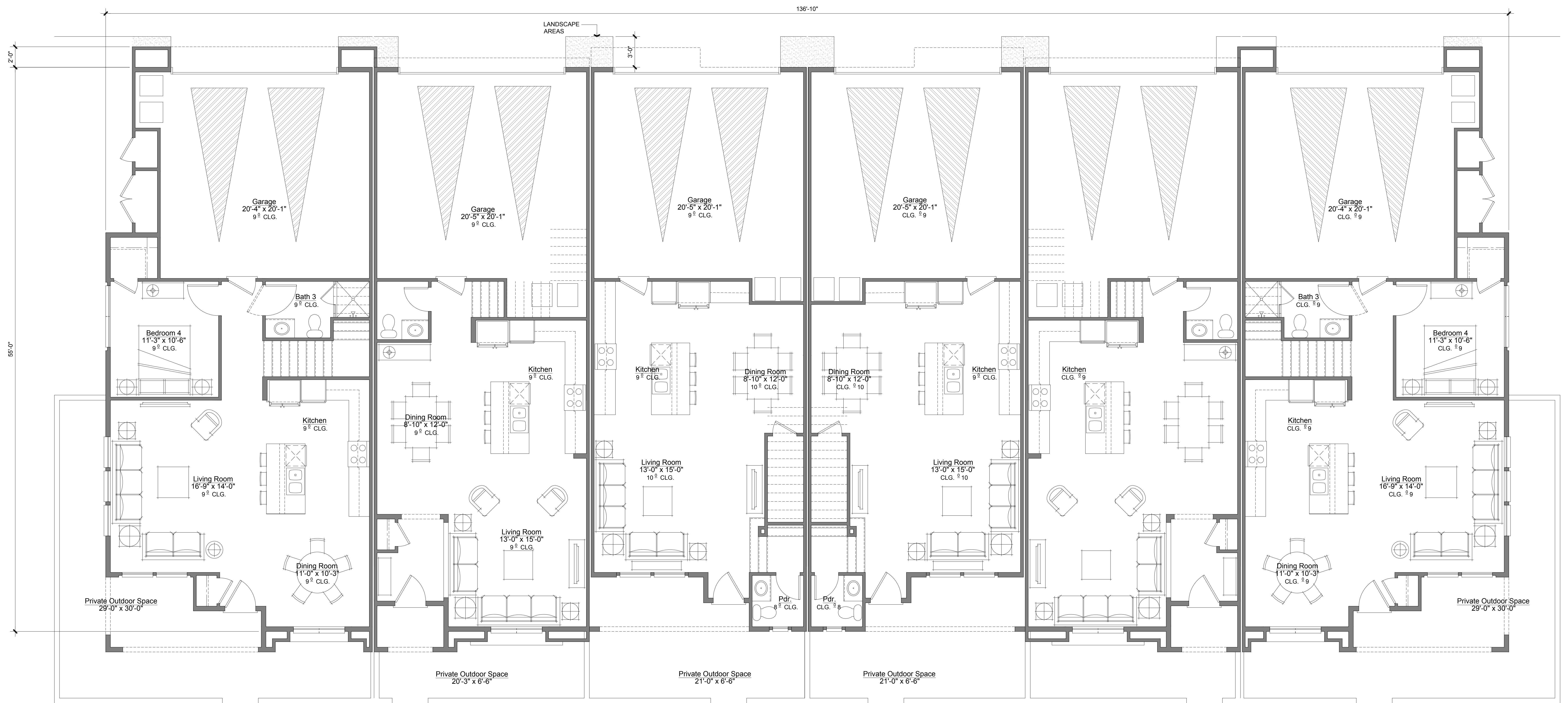
Plan 3 4 Br/3 Ba 1,914 NSF
