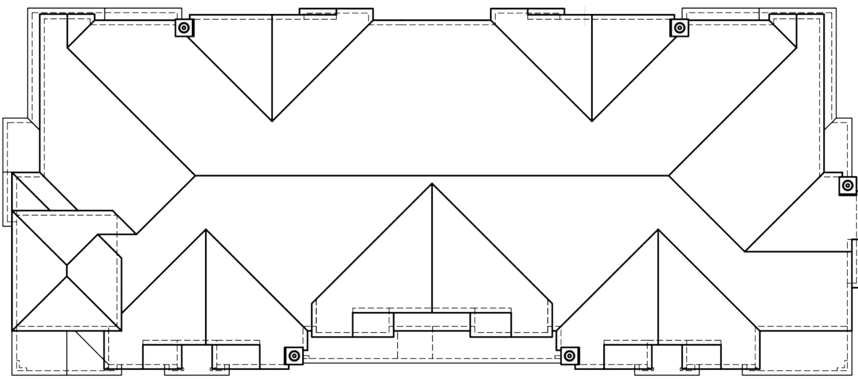
ROOF PLAN 4:12 PITCH EAVE: 12" RAKE: TIGHT
